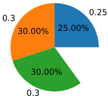
normalize unspecified sum(x) < 1
