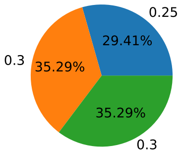
normalize unspecified sum(x) > 1
