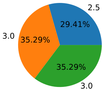
normalize unspecified sum(x) > 1
