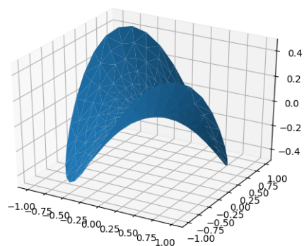
Fig. 13: Trisurf3d
