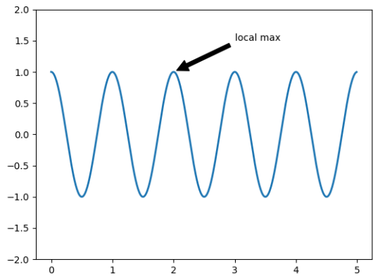
Fig. 23: Annotation Basic
