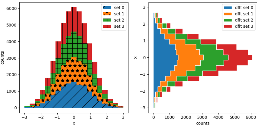
Fig. 28: Filled Step
