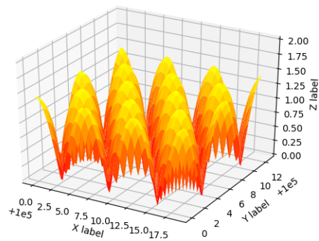
Fig. 11: Offset
