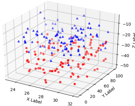
Fig. 81: Scatter3d
