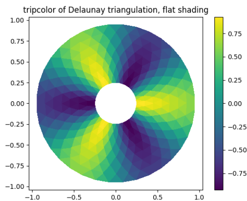
Fig. 16: Tripcolor Demo
