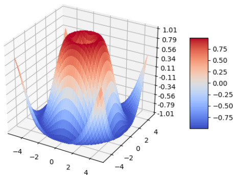
Fig. 7: Surface3d
