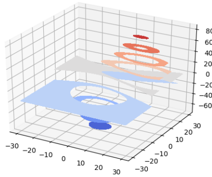
Fig. 86: Contourf3d Contourf3d 2
