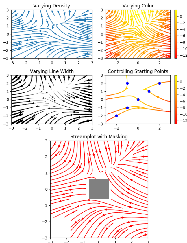
Fig. 15: Plot Streamplot
