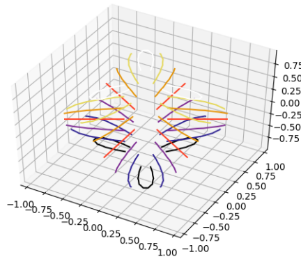
Fig. 19: Tricontour3d
