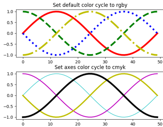
Fig. 26: Color Cycle
