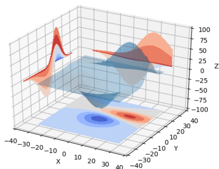
Fig. 12: Contourf3d 2
