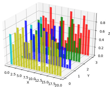
Fig. 88: Bars3d
