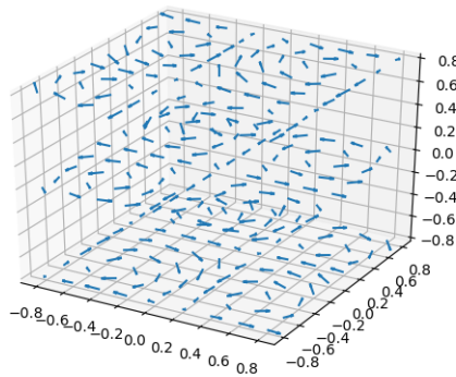
Fig. 25: Quiver3d
