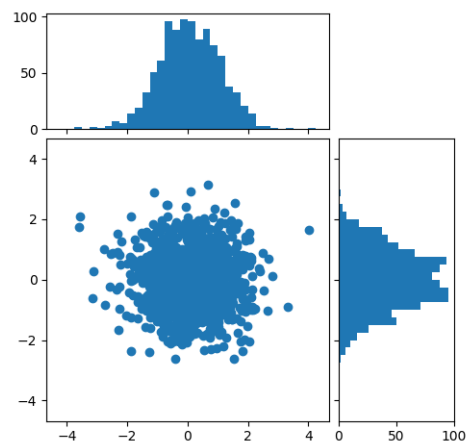
Fig. 53: Scatter Hist
