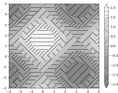
Fig. 17: Contourf Hatching
