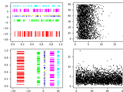
Fig. 20: Eventplot Demo
