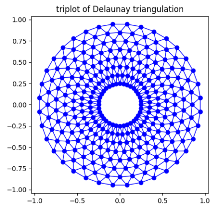
Fig. 7: Triplot Demo
