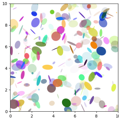
Fig. 9: Ellipse Demo
