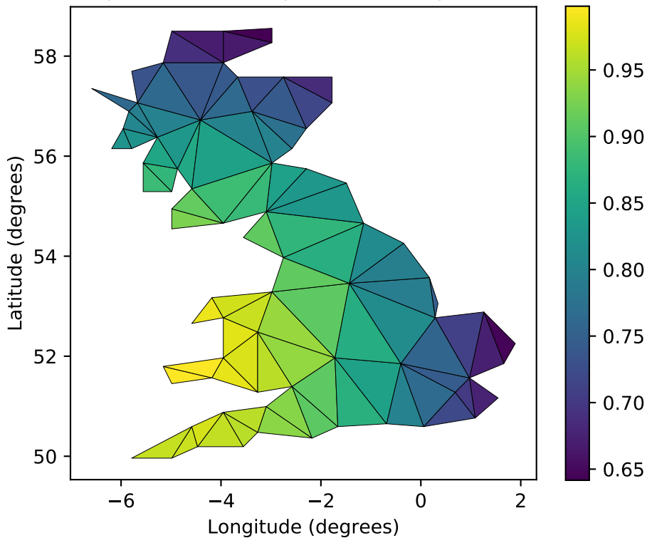
tricolor of user-specified triangulation
