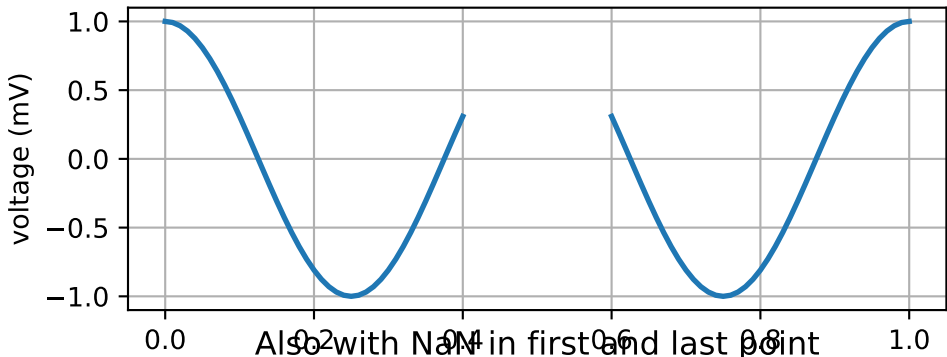
A sine wave with a gap of NaNs between 0.4 and 0.6
