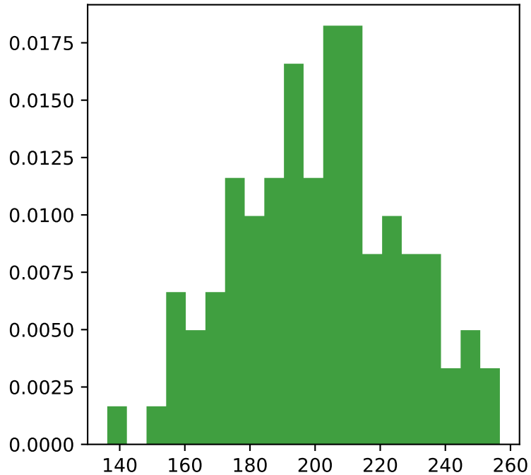
stepfilled
