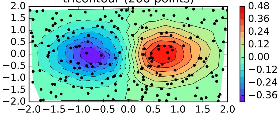
tricontour (200 points)
