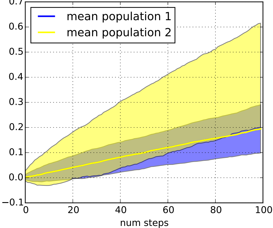
random walkers empirical \mu and \pm\sigma interval
