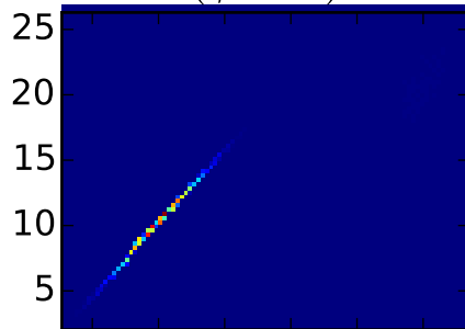
Power law normalization ( \gamma=0.3 )
