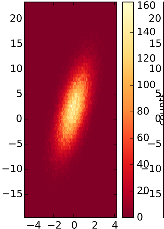
Hexagon binning
