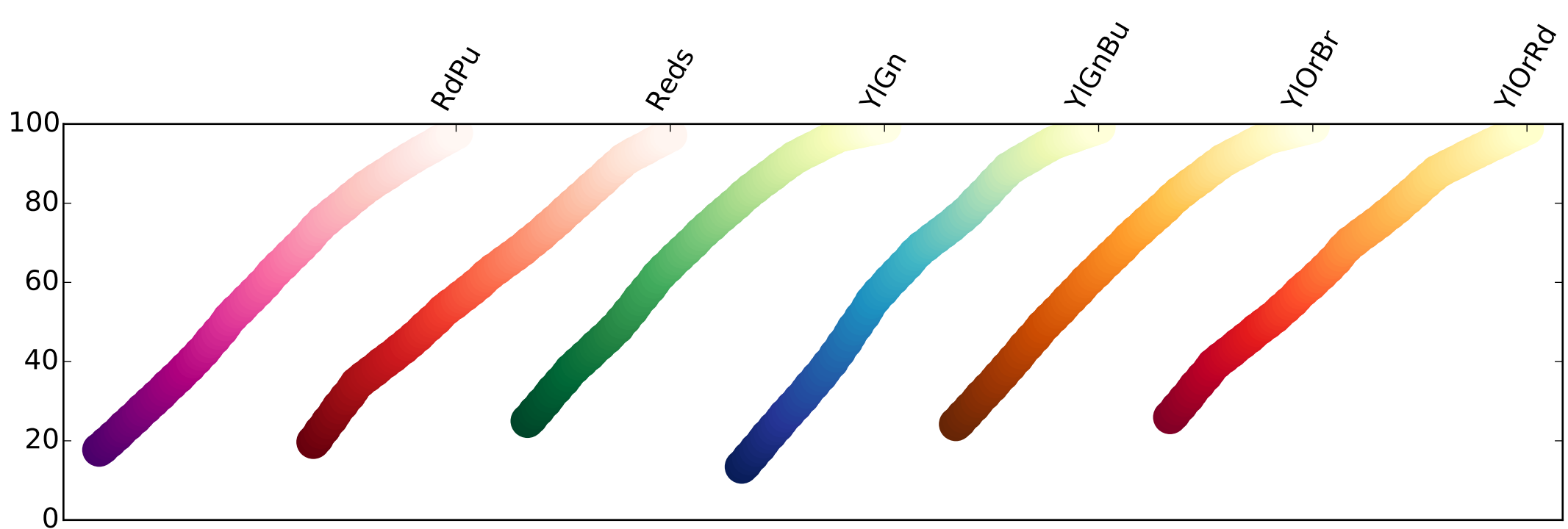
Sequential colormaps
